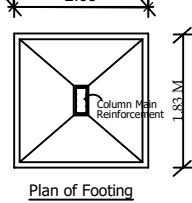
Plan of Footing
