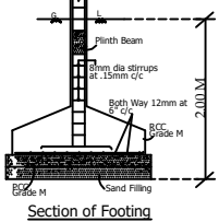
Section of Footing
