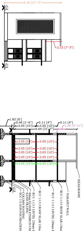
FRONT ELEVATION
