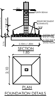
FOUNDATION DETAILS
