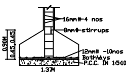
FOOTING DETAILS
