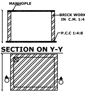
SUMP DETAIL
