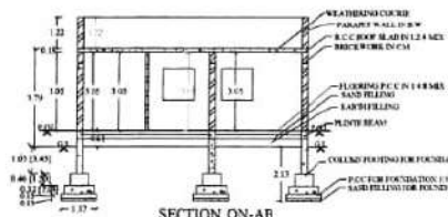
SECTION ON-AB
