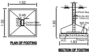
FOUNDATION DETAILS
