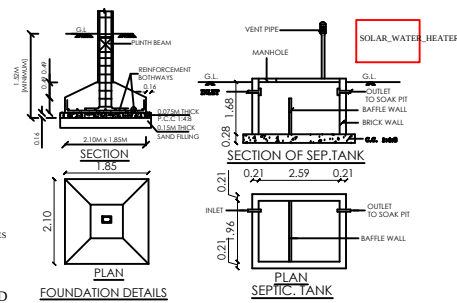
FOUNDATION DETAILS
