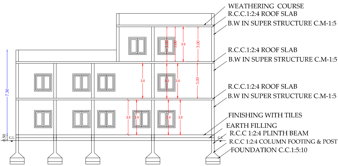
SECTION ON A TO B
