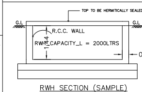
RWH SECTION (SAMPLE
