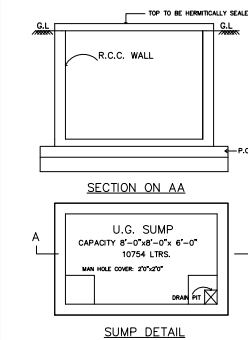
SUMP DETAIL
