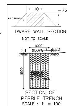
RWH SECTION (SAMPLE
