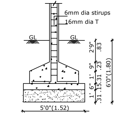
COLUMN FOUNDATION DETAIL
