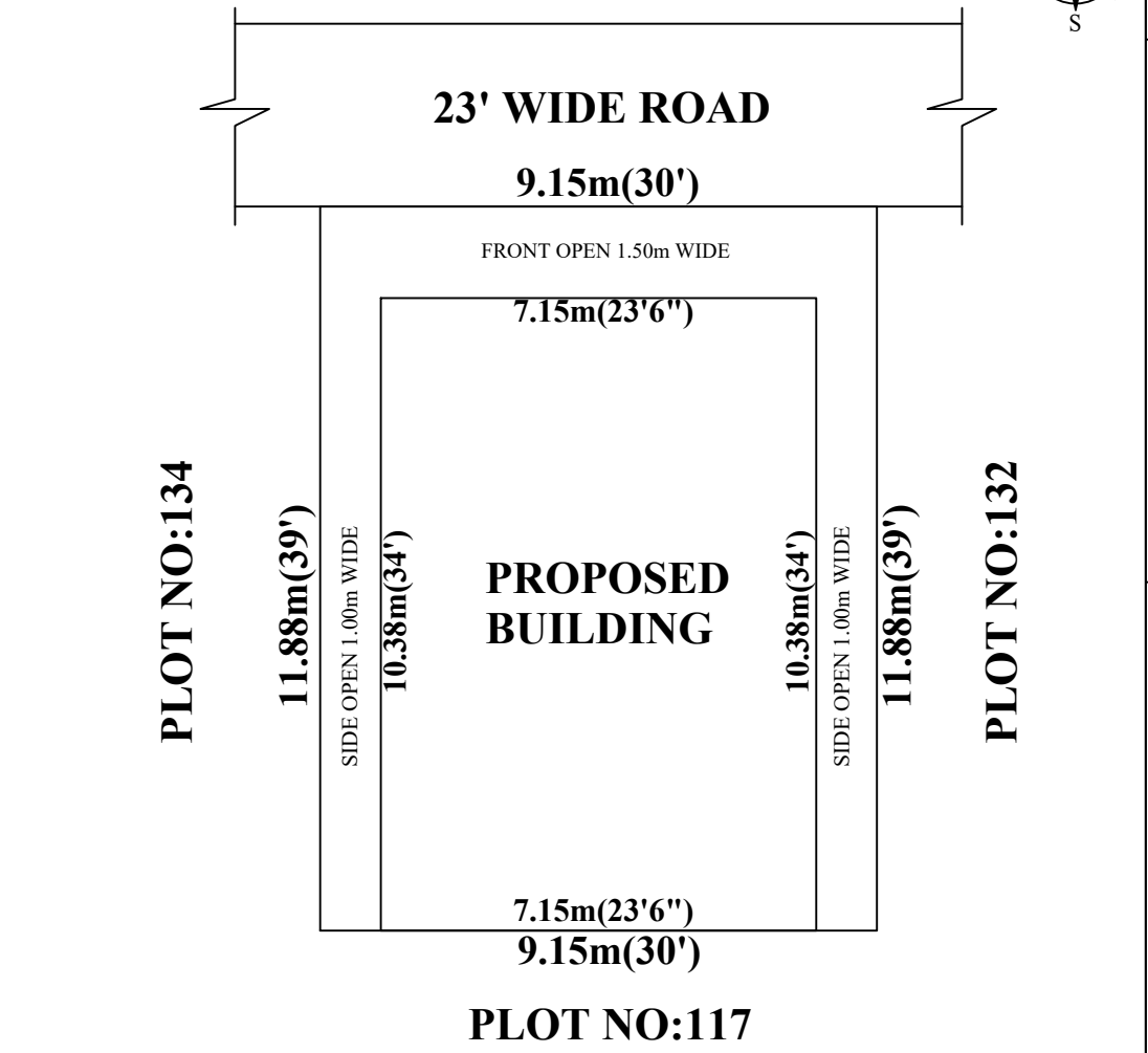
PROPOSED HEAD ROOM FLOOR PLAN
