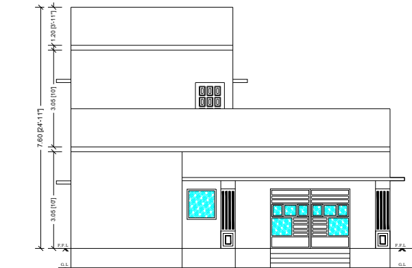
FRONT ELEVATION
