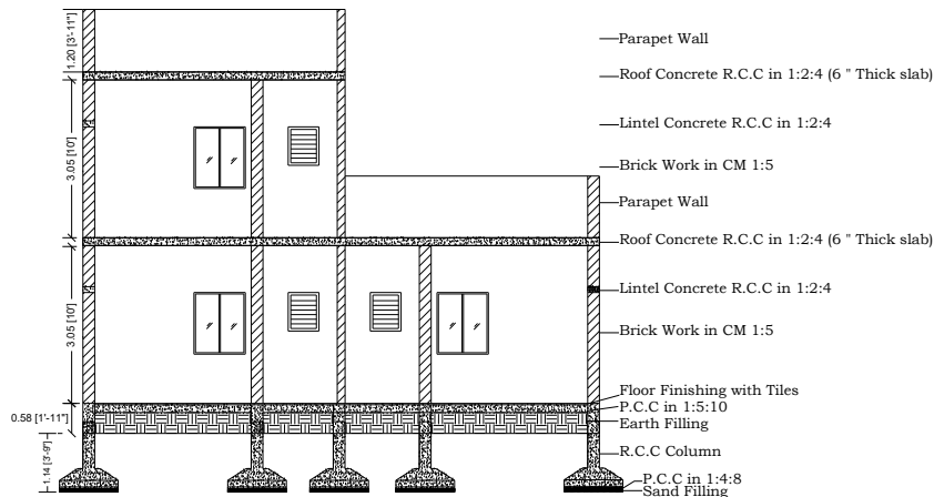
SECTION X-X
