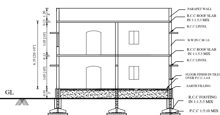
SECTION ON -AAA
