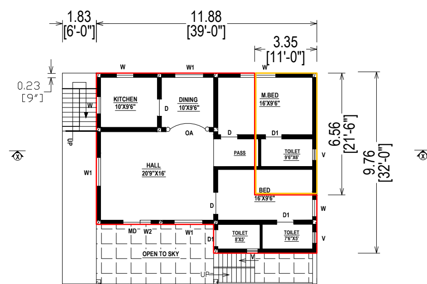
EXISTING & PROPOSED FIRST FLOOR PLAN
