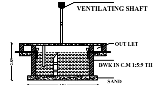
SEPTIC TANK
