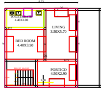
PROPOSED FIRST FLOOR PLAN
