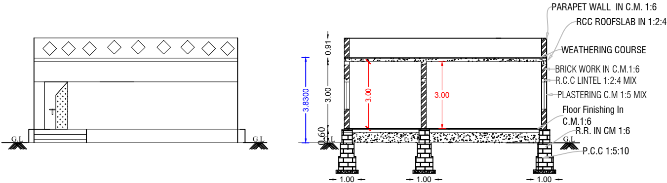
FRONT ELEVATION
