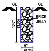
PERCULATION PIT
