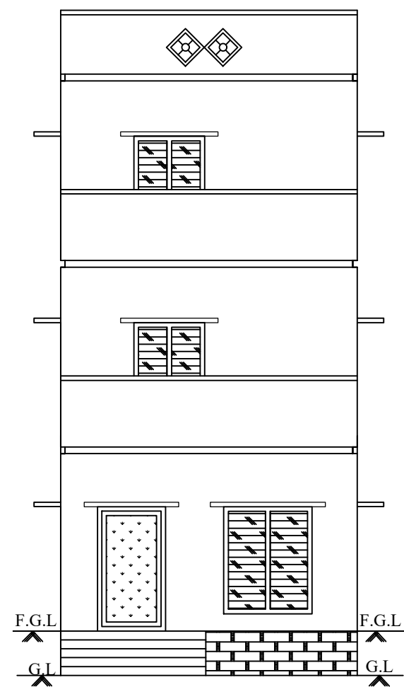
FRONT ELEVATION
