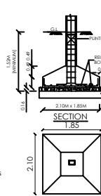
FOUNDATION DETAILS
