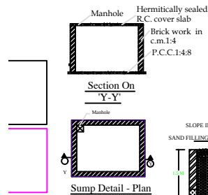
Sump Detail - Plan
