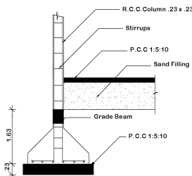
COLUMN DETAIL
