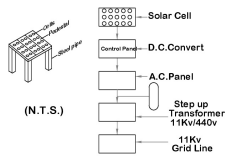
SOLAR SYSTEM FLOW DIAGRAM
