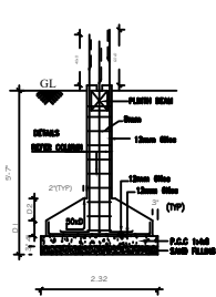
FOUNDATION DETAILS
