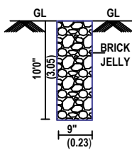
PERCULATION PIT
