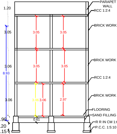
SECTION AB
