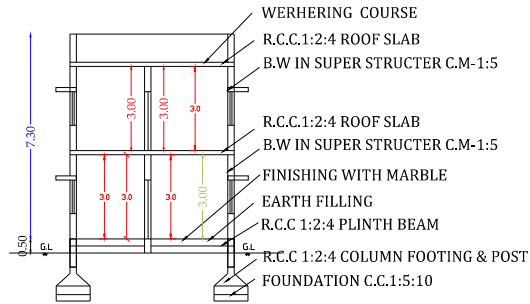
SECTION A TO B
