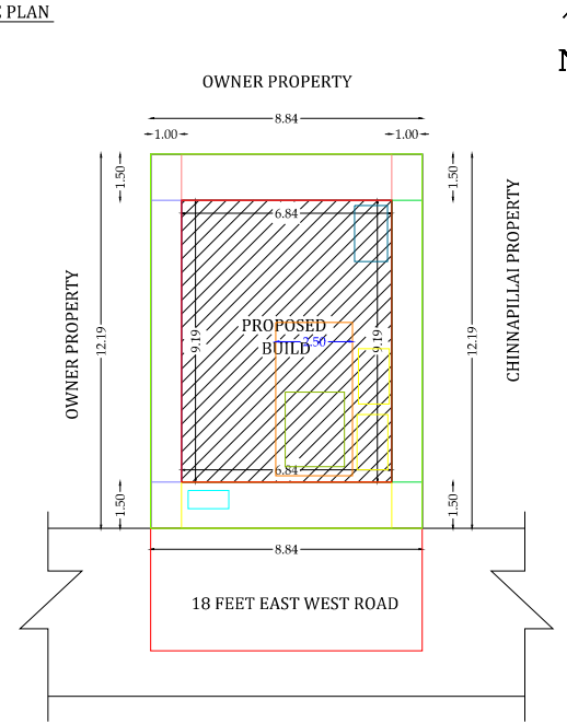
SITE PLAN
