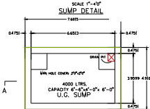
SUMP DETAIL
