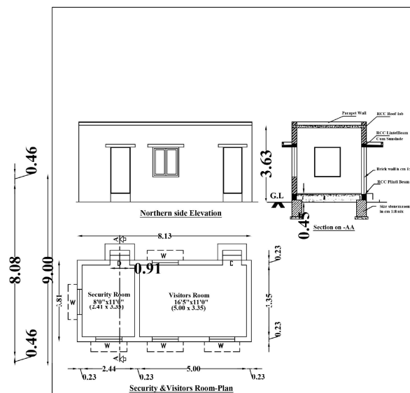
Security & Visitors Room-Plan
