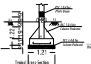
FOOTING DETAILS
