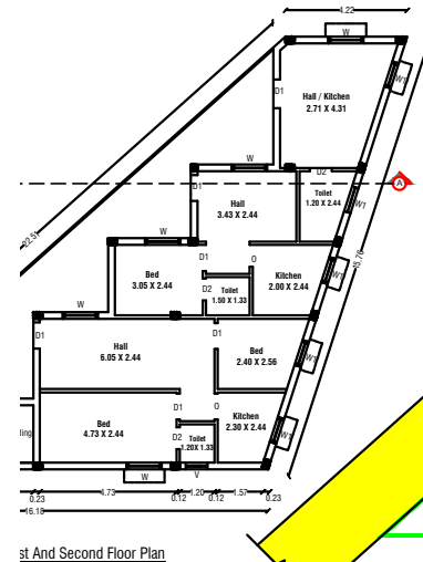
First And Second Floor Plan
