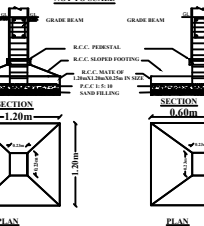
COLUMN FOOTING DETAILS
