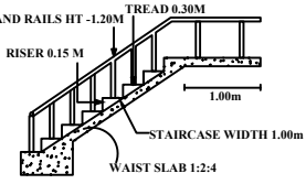
STAIRCASE DETAILS
