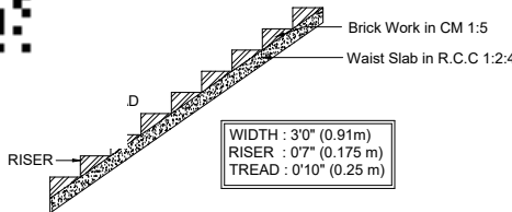
STAIRCASE DETAILS
