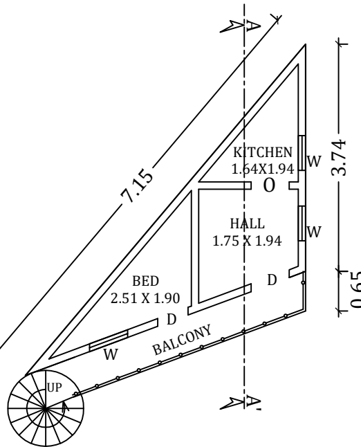
EXISTING APPROVED FIRST FLOOR PLAN
