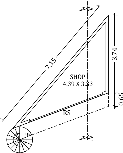
EXISTING APPROVED GROUND FLOOR PLAN
