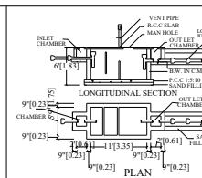
SEPTIC TANK:-
