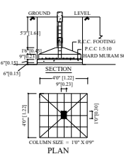
FOUNDATION DETAILS
