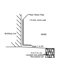
PERCOLATION PIT :
