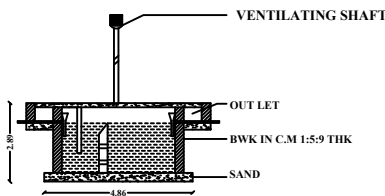
SEPTIC TANK
