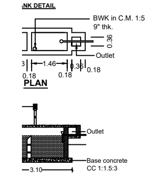
Section of Septic tank
