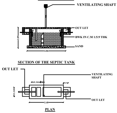
SEPTIC TANK
