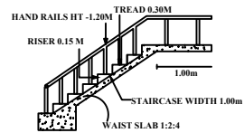
STAIRCASE DETAILS
