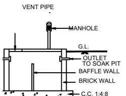
CROSS SECTION OF SEP. TANK
