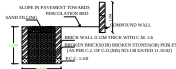
SECTION OF RAIN WATER PERCOLATION BED
