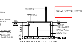
SECTION OF SEPT. TANK
