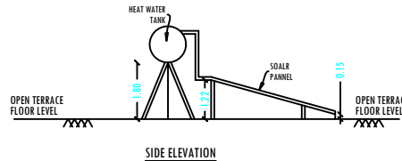
SIDE ELEVATION
