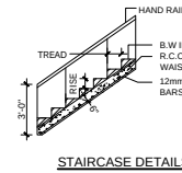
STAIRCASE DETAILS
