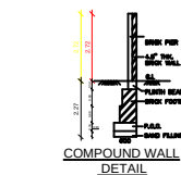
COMPOUND WALL DETAIL
