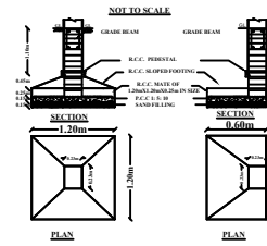
COLUMN FOOTING DETAILS
