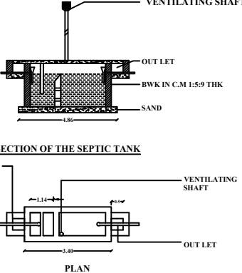
SEPTIC TANK
