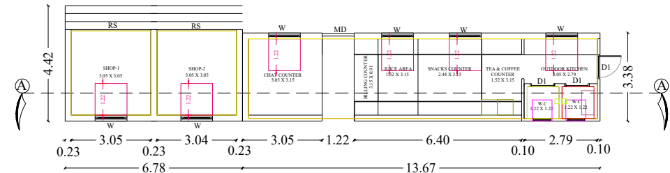
FLOOR PLAN
