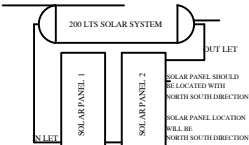
SOLAR WATER HEATER SYSTEM
