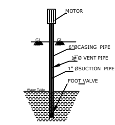
SEC. OF BOREWELL
