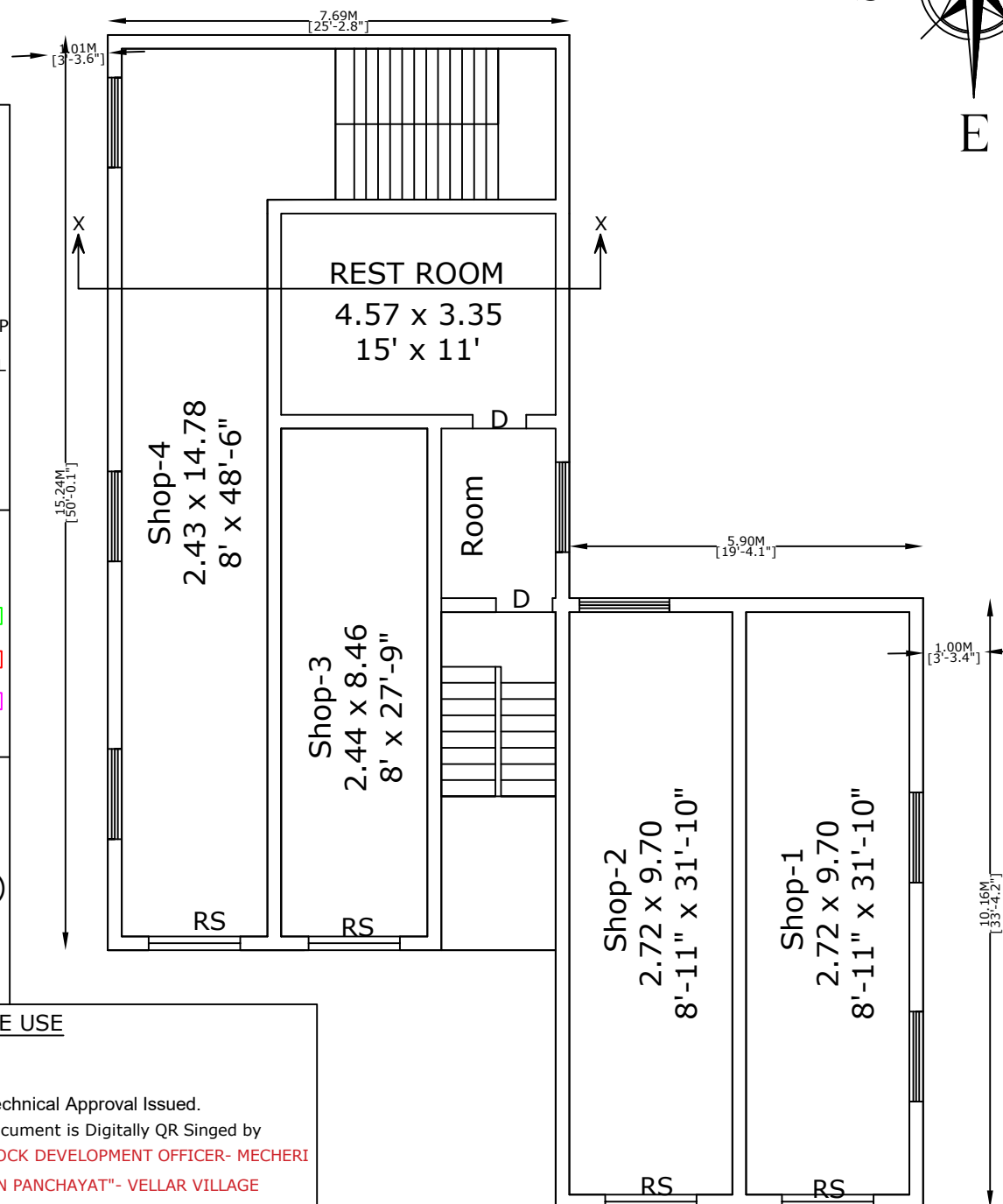
SITE CUM PRO.GROUND FLOOR
