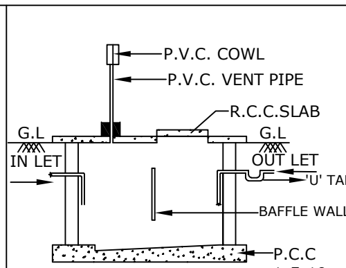
SEC. OF SEPTIC TANK
