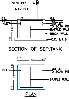
SEPTIC TANK
