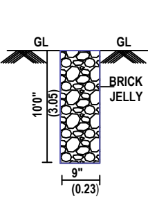
PERCULATION PIT
