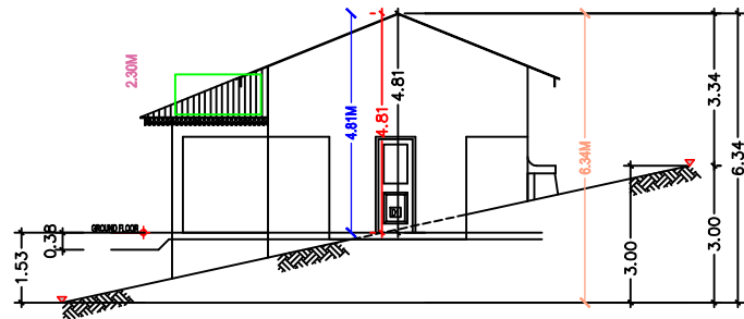
FRONT (WEST SIDE) ELEVATION
