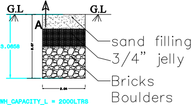
SEPTIC TANK DETAIL
