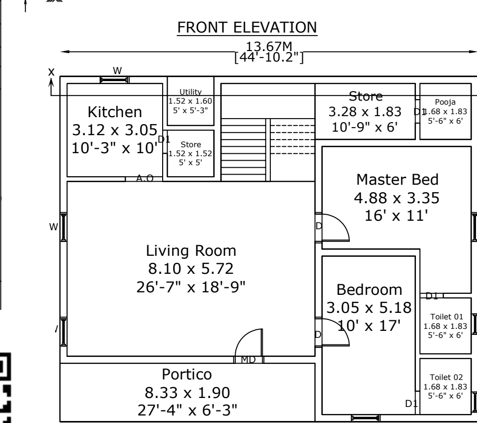
SITE CUM PRO.GROUND FLOOR
