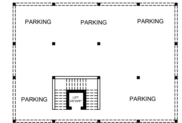
STILT FLOOR PLAN
