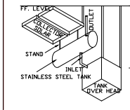
HEATING SYSTEM SOLAR WATER
