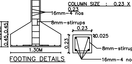
DETAILS OF COLUMNS
