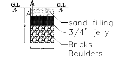
RAIN WATER HARVESTING
