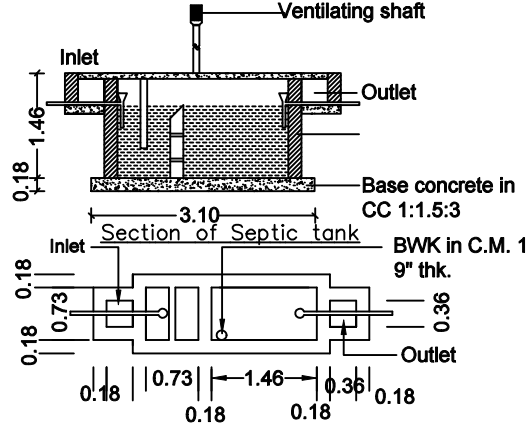
SEPTIC TANK DETAIL
