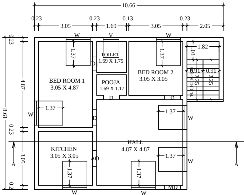
PLAN FOR GROUND FLOOR
