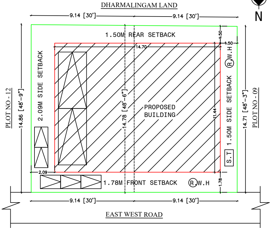
SITE PLAN (1:100)
